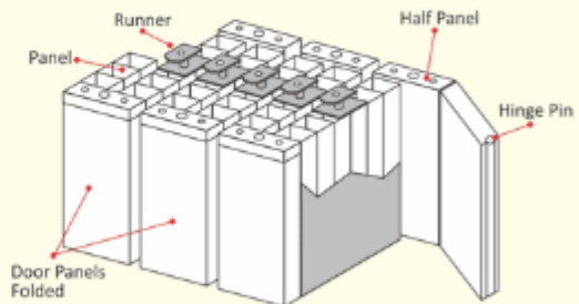
Structure Section A-A
